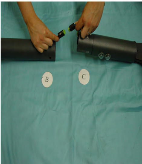
6. Connect the top part of the 993 with the two heaters. Connect the 2 connectors, run in the cable and insert pole B in pole C. Tighten the 4 6MA socket head screws, positioning and then tightening them. At this point the heater is ready for use.
